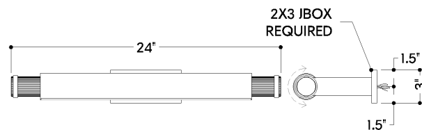
FRONT
