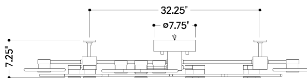
FRONT
