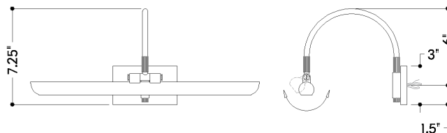
FRONT
