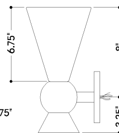
SIDE
